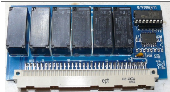
SMD-Version
